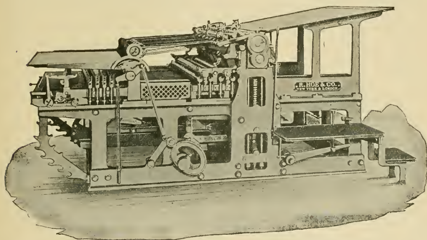
FOUR ROLLER TWO-REVOLUTION PRESS.
